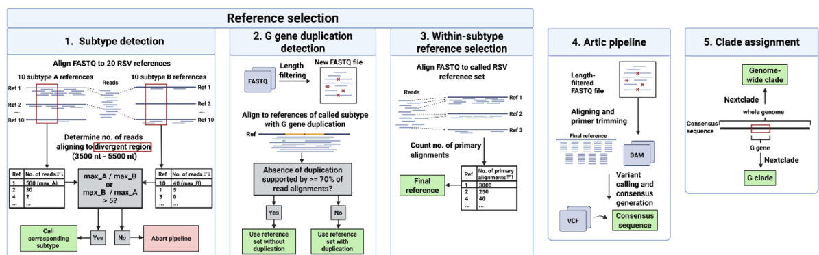
Fig. 4. Computational workflow. The first three steps were performed to select the reference which resembles the isolate the most. The subtype and the presence of the G gene duplication were first detected. Then, from a subset of references with corresponding features, the final reference was selected. Consensus sequences were then generated using the ARTIC pipeline and G clade and genome-wide clades were called using Nextclade.
