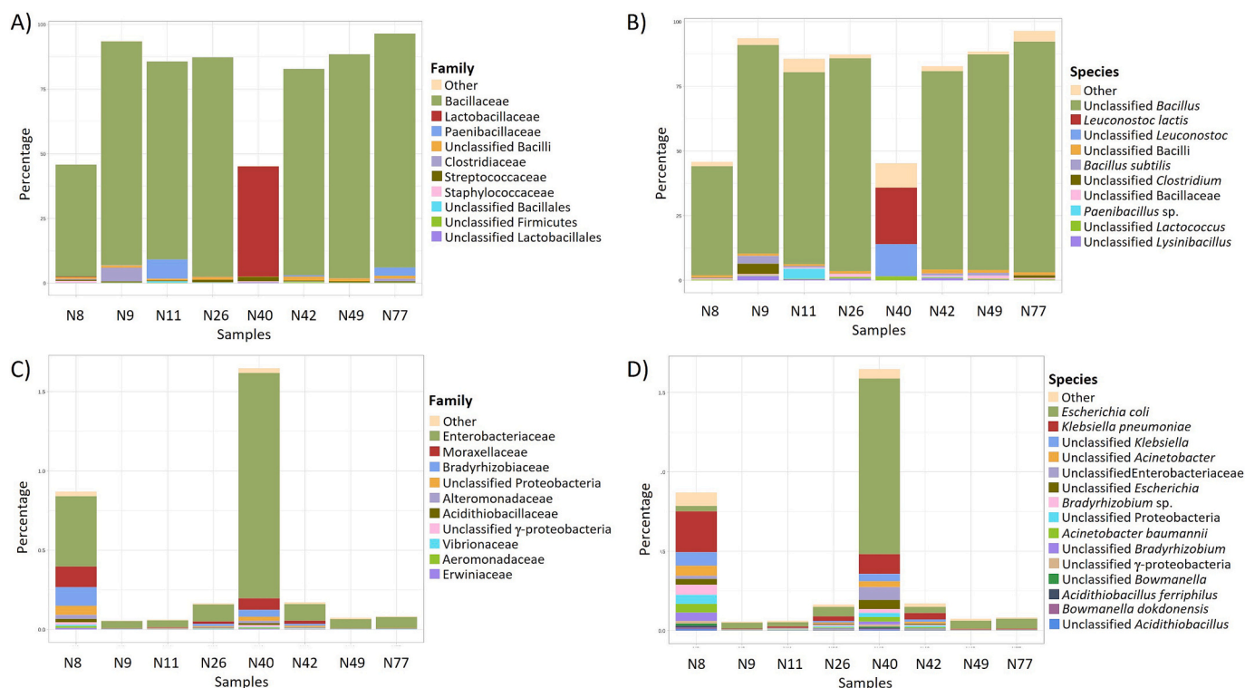
Fig. 1. Main microorganisms detected by metagenomic analysis of frozen chicken nuggets. Panels A and B correspond to microbial families and species belonging to the phylum Firmicutes, respectively; Panels C and D correspond to microbial families and species belonging to the phylum Proteobacteria, respectively. Samples N8 and N9 (brand B), N11 and N42 (brand A), N40 (brand C), and N49 (brand D) yielded bacterial growth on MacConkey (i.e.: Gram-negative bacilli); samples N26 and N77 (brand B) only yielded growth on TSA plates.
