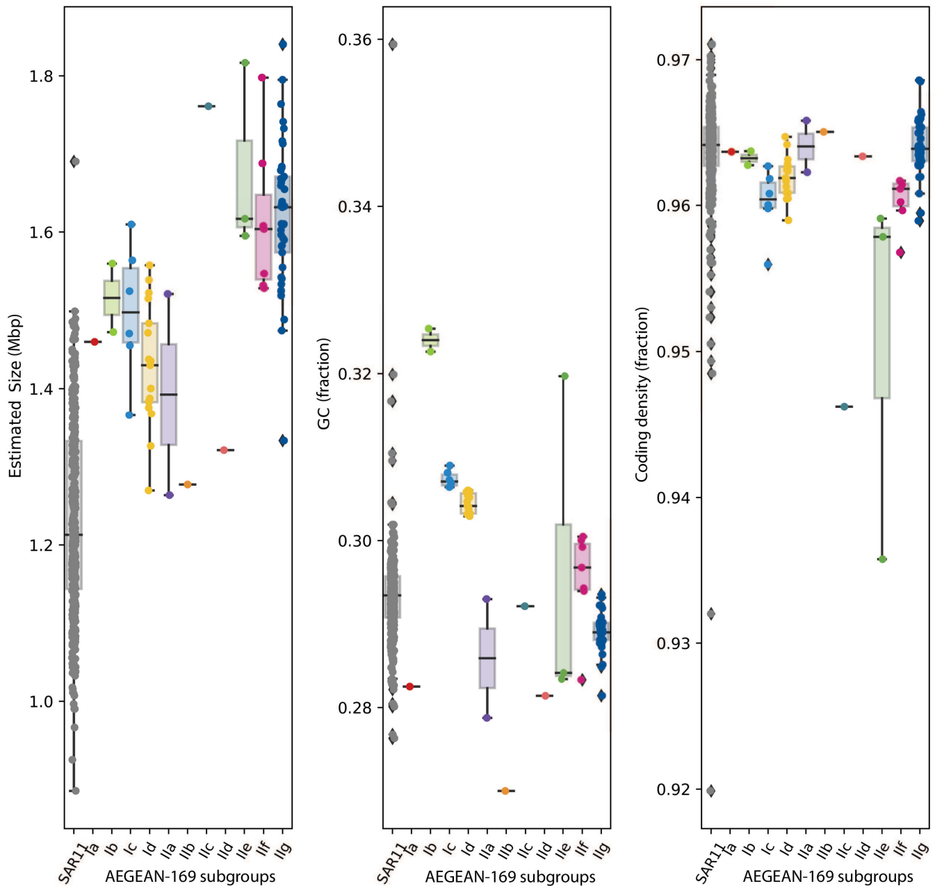
FIG 2 Boxplots illustrating the bulk genome characteristics of AEGER-169 subgroups compared to SAR11. Subgroups are colored according to the tree in Fig. 1 and denoted on the x-axis. Boxes describe the interquartile range (IQR) with the median indicated as a bar. Whiskers indicate 1.5x IQR, and outlier points are plotted beyond the whiskers. The underlying data points are also plotted on top of each boxplot.
