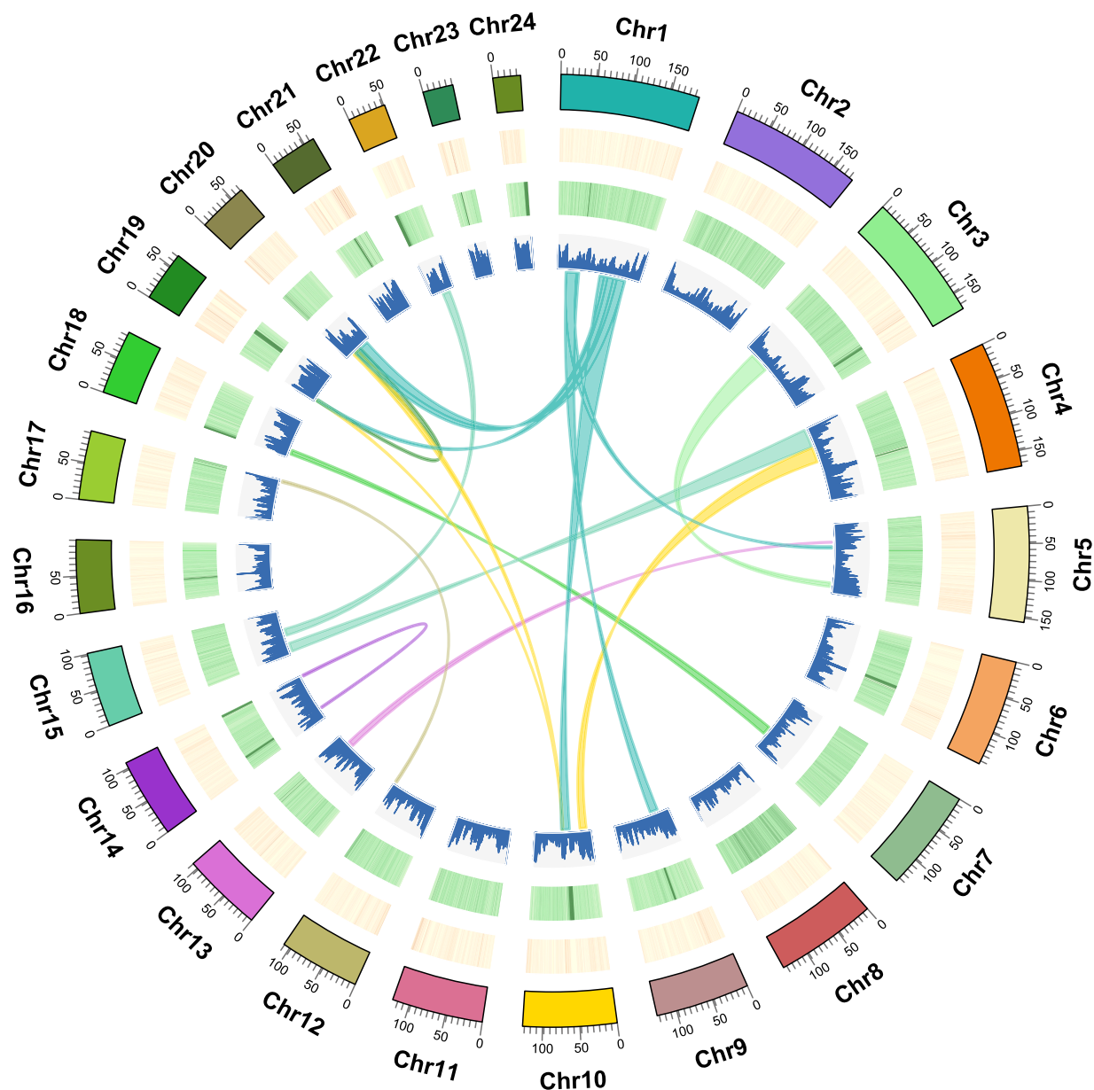
Fig. 3 Collinearity of the Yarkand hare assembled genome. From the outside in: first circle, chromosomes; second circle, gene density (window = 100 kb); third circle, REPEAT density (window = 100 kb); fourth circle, GC content (window = 100 kb); inside, covariance within the genome obtained using MCSanX gene block analysis.
