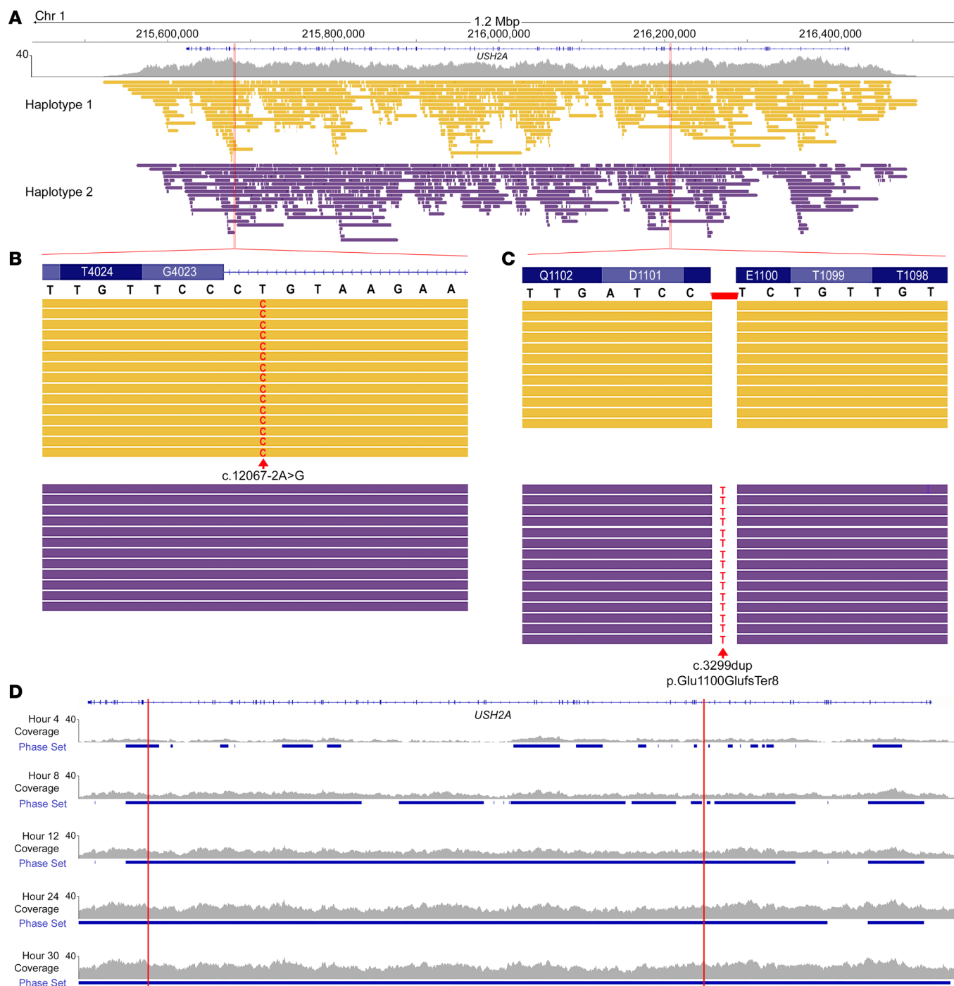
Figure 5. Targeted panel genome sequencing allows for rapid identification of disease-causing variants. (A) In an affected individual with no prior genetic testing, targeted long-read panel sequencing revealed 2 likely disease-causing variants in the USH2A gene, (B) an SNV noted to be pathogenic, and (C) a duplication leading to a frameshift and early termination that was in trans . (D) Post hoc analysis of the sequencing data revealed that the 2 variants in USH2A were identified and properly phased within 12 hours of sequencing, whereas the entire USH2A gene could be phased 30 hours after sequencing.
