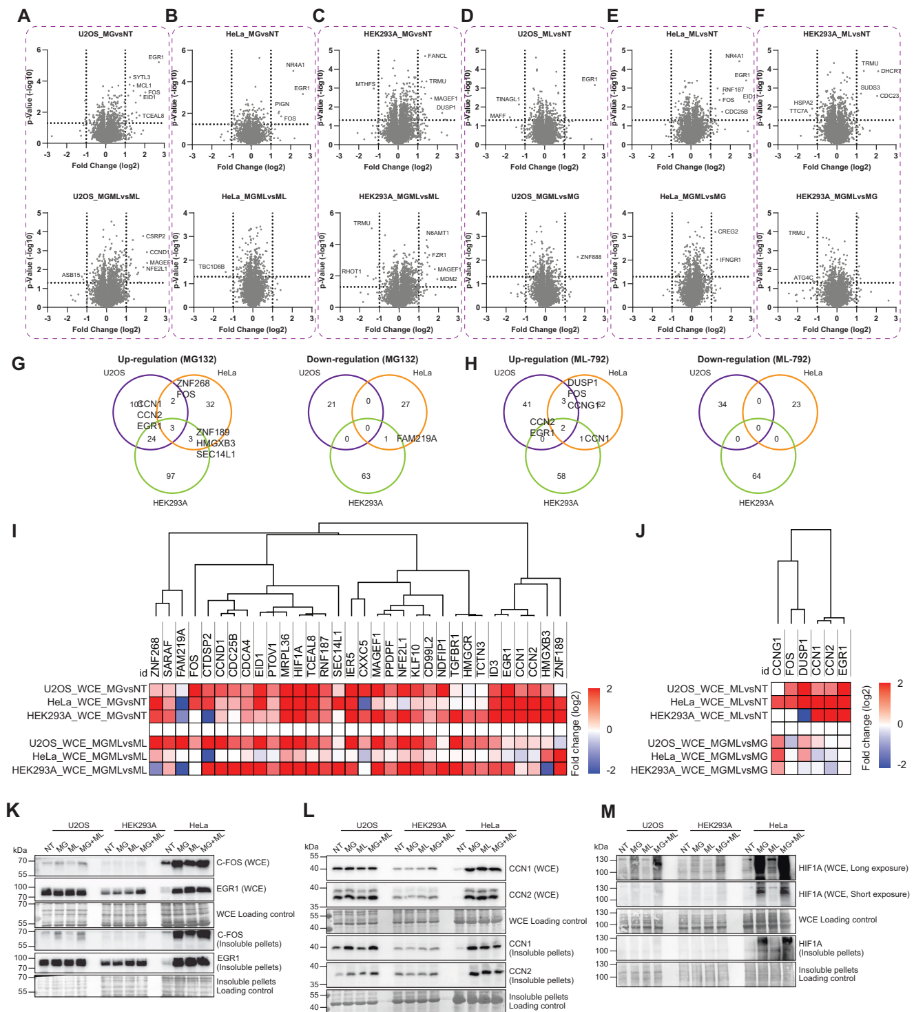
Fig. 3 | Drug-induced modulation of protein levels. Volcano plots showing the comparisons of protein levels between MG132 vs vehicle, and MG132 + ML-792 vs ML-792 from (A) U2OS, (B) HeLa, and (C) HEK293A cells. Volcano plots showing the comparisons of protein levels between ML-792 vs vehicle, and MG132 + ML-792 vs MG132 from (D) U2OS, (E) HeLa, and (F) HEK293A cells. P -values were calculated using a two-tailed Student's t -test. No adjustments for multiple comparisons were applied. G Venn diagram showing the overlaps of up- and down-regulated proteins obtained from three cancer cell lines following treatment of MG132. Differentially regulated proteins from two pairwise comparisons of MG132 vs vehicle and
