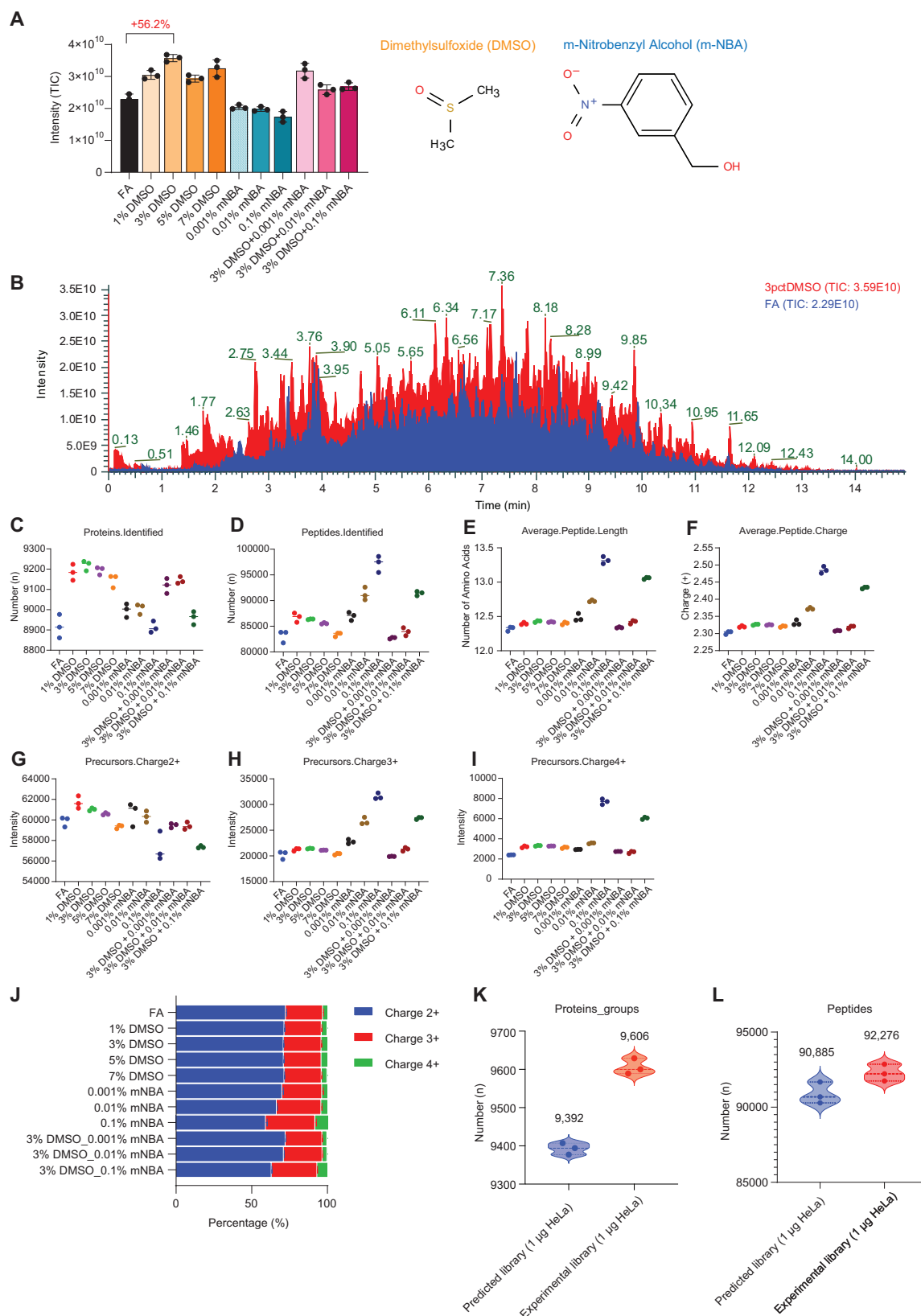
Fig. 1 | Evaluation of the effect of supercharging mobile phase modifiers in nDIA proteomics. A The TIC intensities obtained with different composition of LC solvents. B Example of TIC profiles obtained with or without 3% DMSO. (C) Identified proteins, (D) identified peptides, (E) average peptide length, (F) average peptide charge, (G) number of peptides with 2+ charge state, (H) number of peptides with 3+ charge state, and (I) number of peptides with 4+ charge state obtained with different composition of LC solvents, (J) distribution of peptide charge states
