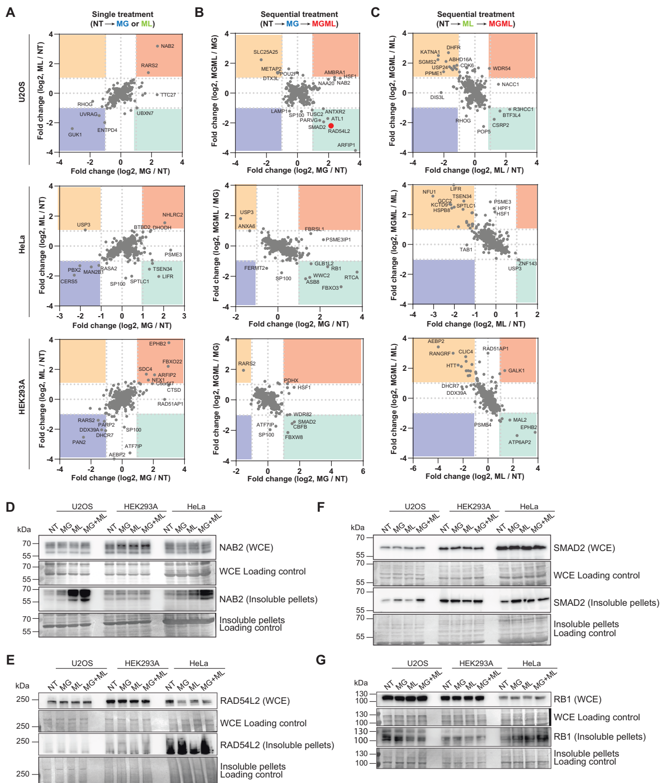
Fig. 6 | Combinational effects of MG132 and ML-792 on protein solubility.
