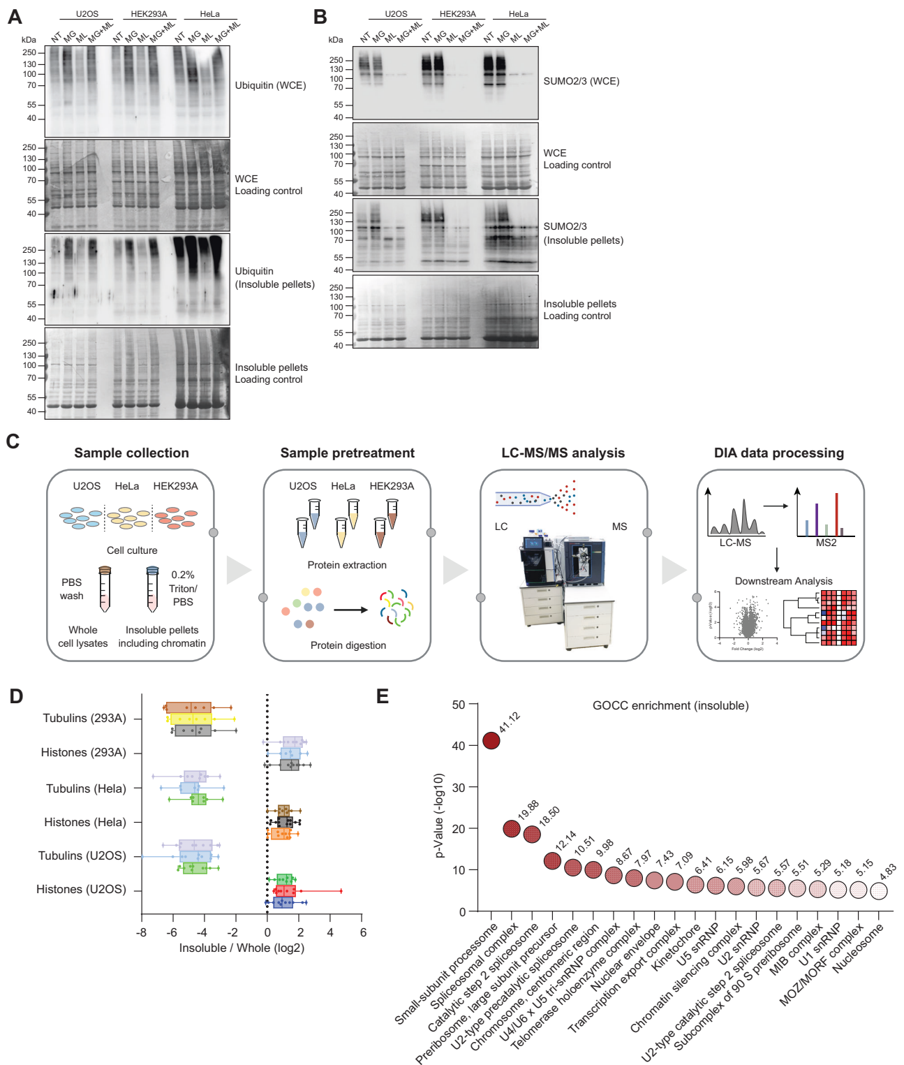
Fig. 2 | Overview of proteome-wide solubility shift proteomics. Western blotting result of Ubiquitin ( A ) and SUMOs ( B ). Experiments were repeated at least three times, and similar results were obtained. ( C ) Schematic of the sample preparation, MS data acquisition, and data processing workflow of solubility shift proteomics. D MS intensity changes of histones and tubulins identified in three cancer cell lines. Only samples without drug treatment are displayed. Three biological replicates were used for each sample group. Scatter points represent the \log_2 enrichment ratios of identified histone ( n = 14 ) or tubulin ( n = 15 ) isoforms in the insoluble fraction relative to whole-cell lysate. Box plots show the median (center line), the
