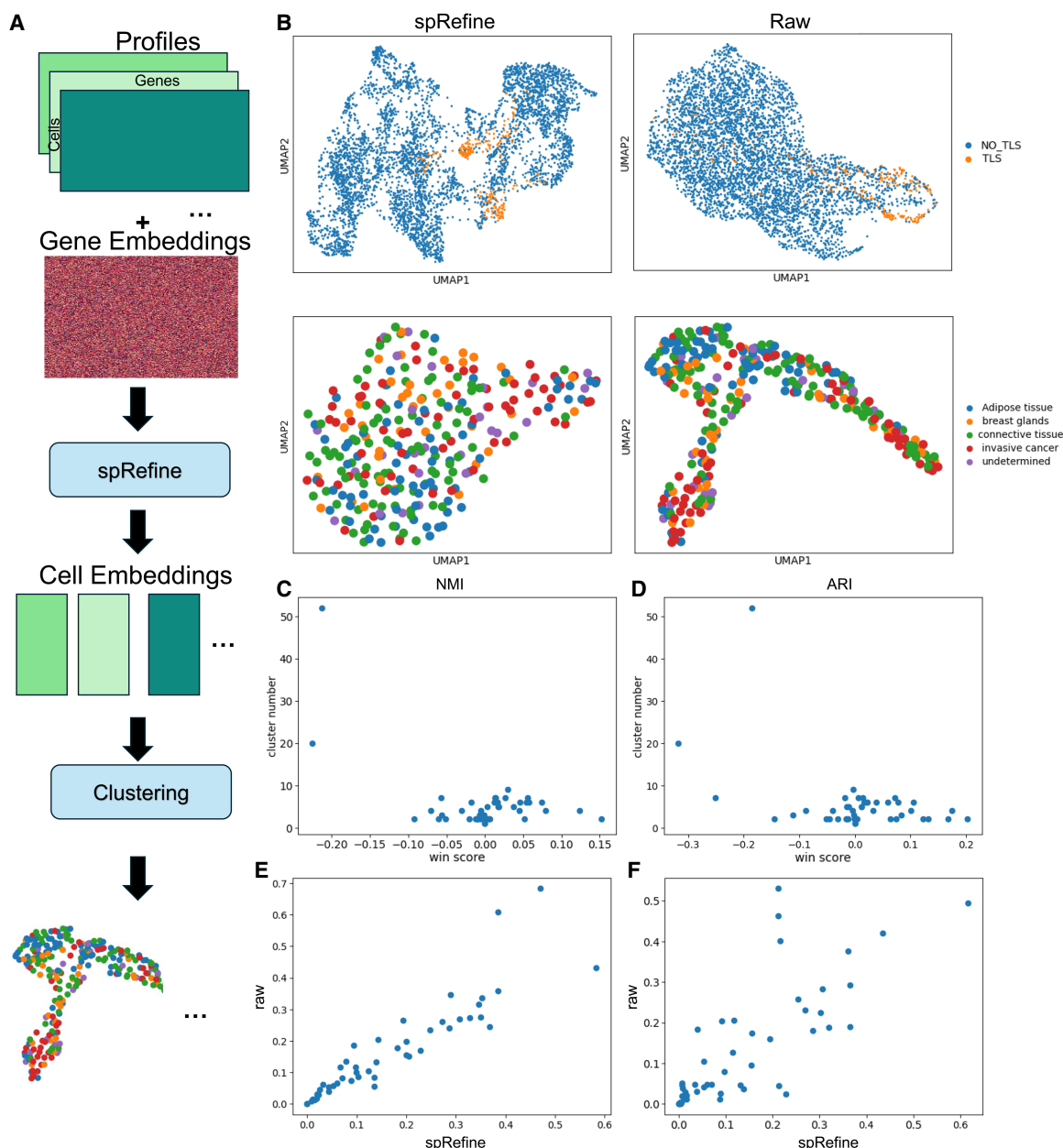
Figure 4. Analyzing the results of spRefine pretrained with large-scale spatial transcriptomics. (A) The workflow of pretraining spRefine for phenotype-level identification. (B) The UMAPs for visually comparing spot representations before ( right ) and after ( left ) imputation based on the two selected samples with different cell states. (C) The relationship between win rate computed based on NMI and cluster number. (D) The relationship between win rate computed based on ARI and cluster number. (E) The relationship between the NMI scores of raw data and data imputed by spRefine. (F) The relationship between the ARI scores of raw data and data imputed by spRefine.
