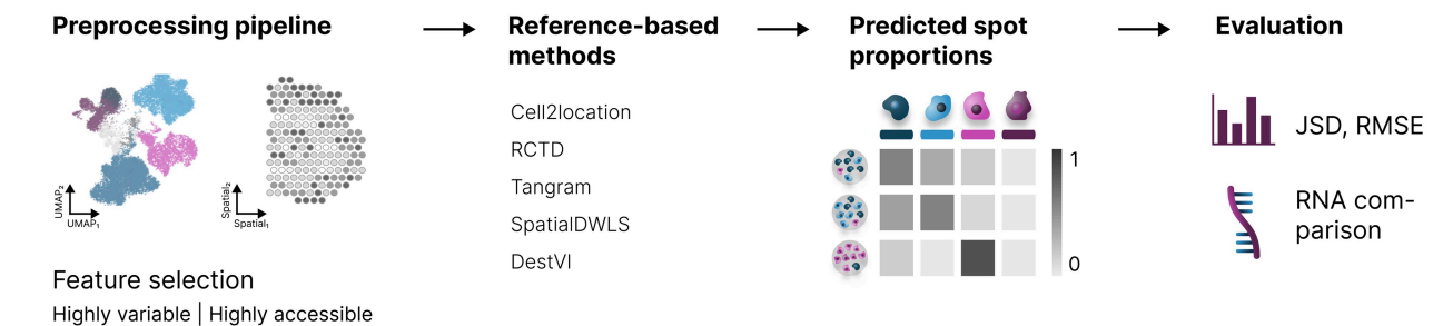
Figure 1. Workflow for evaluating spatial deconvolution methods developed for spatial transcriptomics data on spatial chromatin accessibility data. (a) Spatial deconvolution has been developed and successfully applied to spatial transcriptomics data at spot resolution to decompose the cell-type composition in individual spots. We evaluate deconvolution methods originally designed for transcriptomics measurements on their capabilities to deconvolve spatially-resolved chromatin accessibility data. We provide a framework to simulate spatial epigenetic data in two ways: (b) through the silver standard by leveraging dissociated references and c, through the gold standard by leveraging targeted spatial ATAC datasets. Our pipeline allows the generation of spot-based data with different cell densities, cell-type heterogeneity, and spatial distributions to accurately reflect tissue patterns observed in real datasets (b). Epigenetic information measured with targeted technologies can be aggregated to spot-based spatial data by aggregating features overlapping artificial spots (c). (d) The benchmarking pipeline incorporates different feature selection strategies and tests five deconvolution methods: Cell2location, RCTD, Tangram, SpatialDWLS, and DestVI. Performance is evaluated based on two different metrics: RMSE and JSD. Additionally, we compare the performance obtained on spatial transcriptomics measurements. Heart and brain icons were created in BioRender. Heumos, L. (2025) https://BioRender.com/d08u1k8 .
