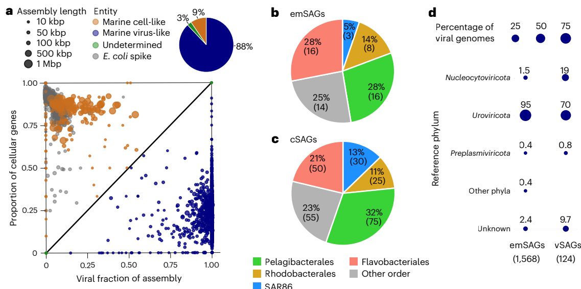
Fig. 2 | Compositional overview of de novo genome assemblies obtained from coastal seawater using EMCG and other methods. a, The fraction of prokaryotic genes relative to the fraction of virus-like sequence length in individual genome assemblies, which was used to tentatively distinguish cellular (orange) and virus-like (blue) SAGs. The SPCs containing E. coli cells were included in the EMCG workflow as internal standards (grey). The pie chart summarizes the
