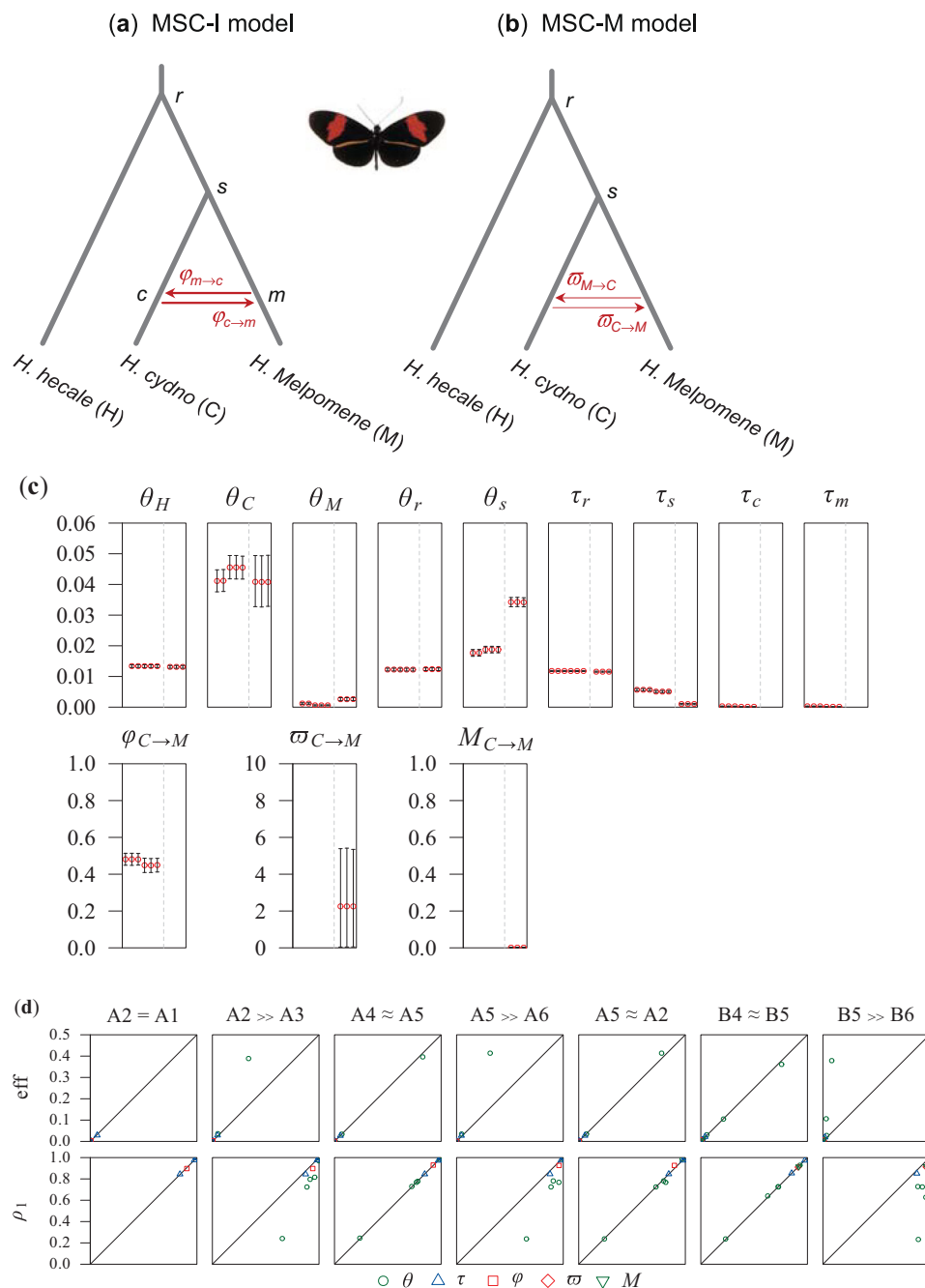
Fig. 7 | Analysis of the Heliconius dataset. a MSC-I and b MSC-M models for three Heliconius species: H. hecale (H), H. cydno (C), and H. melpomene (M), with potential gene flow between H. cydno and H. melpomene . Models with the C \rightarrow M gene flow are used to analyse genomic sequence data. Picture of Heliconius melpomene
