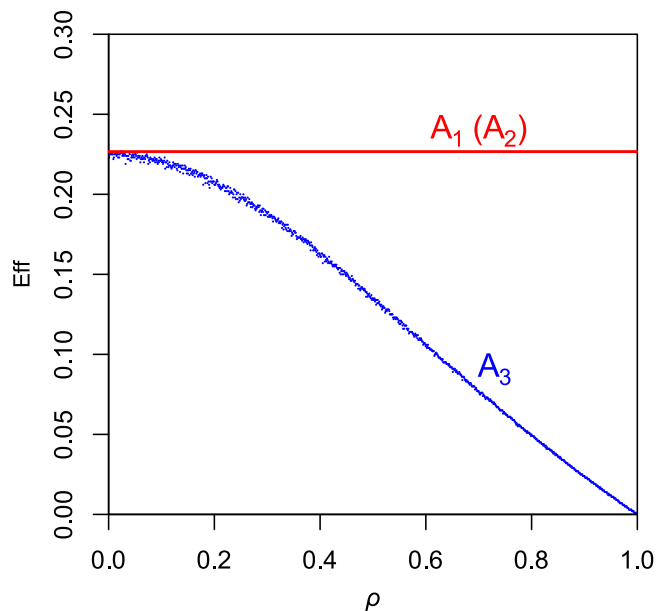
Fig. 4 | Efficiency for three MCMC algorithms in a bivariate Gaussian target. Efficiency for estimating \mu_x in the N_2 target of eq. (17) is measured by E of eq. (15). In algorithm A1, y is integrated out and a sliding-window move is used to sample x from its marginal. This has the same efficiency as algorithm A2, which samples y' from its conditional for the newly proposed x' : \pi(y'|x') . Note that E does not depend on \rho for A1 and A2. In Algorithm A3, two one-dimensional sliding-window moves are used to update x and y , respectively. Efficiency is calculated for 1000 values of \rho by running the algorithm over 10^7 MCMC iterations. A3 suffers from the correlation between x and y : E = 0.228 at \rho = 0 (equivalent to A1 and A2) but drops to 0.024 at \rho = 0.9 and 0.012 at \rho = 0.95 .
