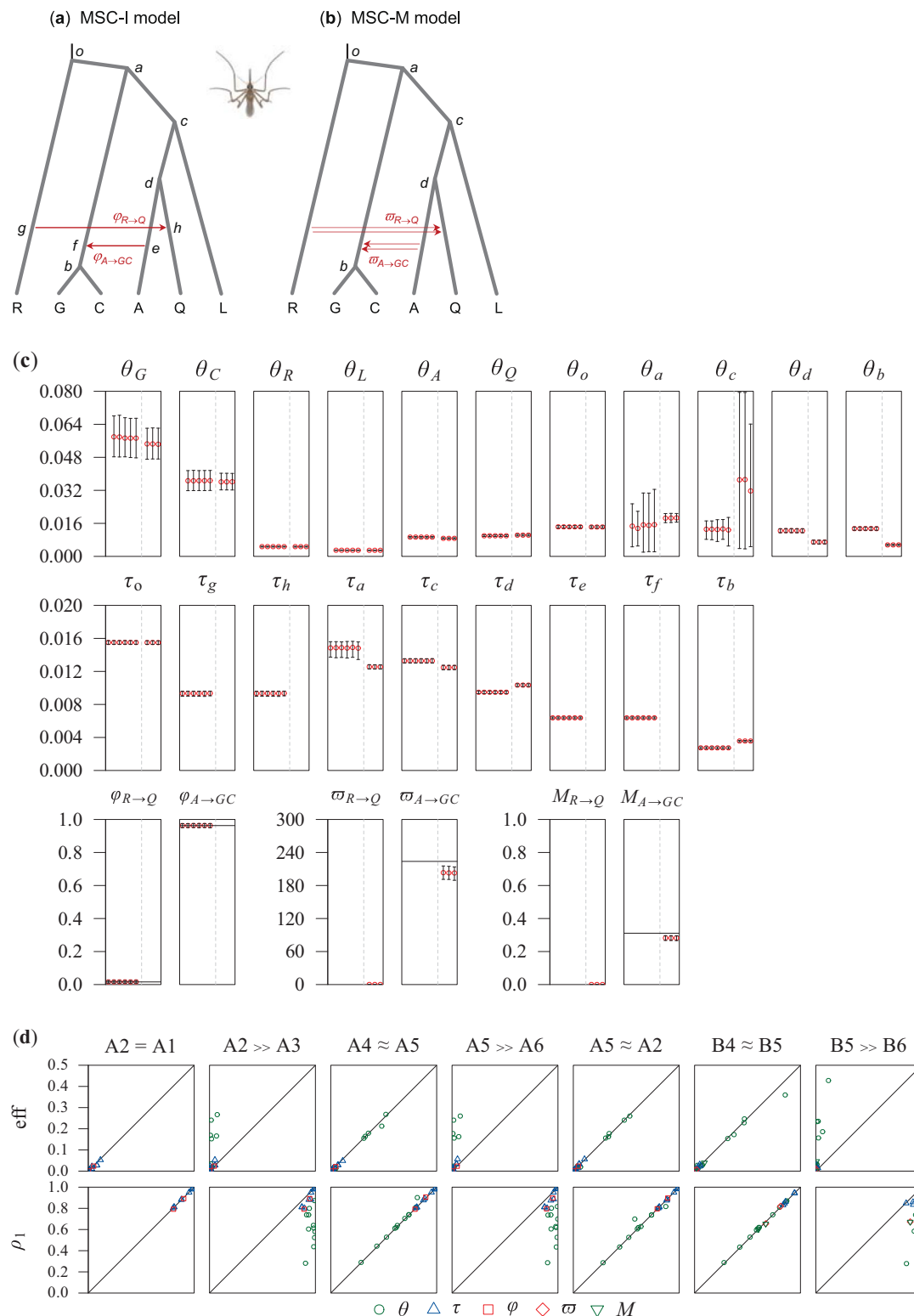
Fig. 6 | Analysis of the Anopheles mosquito dataset. a MSC-I and b MSC-M models for six species of African mosquitoes in the Anopheles gambiae species complex: A. gambiae (G), A. coluzzii (C), A. arabiensis (A), A. melas (L), A. merus (R), and A.
