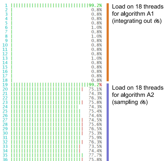
Fig. 8 | Screenshot for the htop command showing the CPU load for algorithms A1 (integrating out \theta s) and A2 (sampling \theta s from their conditionals) applied to the Adansonia dataset under the MSC-I model (Fig. 5a). The two algorithms were run on two CPUs in the sameserver, each using 18 threads, taking 5 \times 10^5 samples after a burn-in of 5 \times 10^4 . With algorithm A1, all MCMC steps including the gene-tree node age and gene-tree SPR proposals are conducted serially (although likelihood calculation is parallelised by loci), so that the main thread has CPU usage close to 100% while the worker threads spend most time waiting with low CPU usage of \leq 1\% . With algorithm A2, the gene-tree node age and gene-tree SPR proposals are conducted in parallel so that the worker threads achieve high CPU usage of \sim 75\% . Running time was 43h15m for A1 and 5h18m for A2, with an 8.2-fold speedup.
