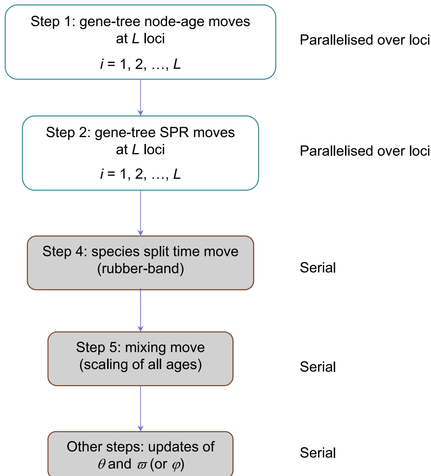
Fig. 3 | MCMC proposal algorithms implemented in BPP. Species split times (step 4) are updated one after another, and within each calculations of the gene-tree density and likelihood for all loci are executed in parallel.
