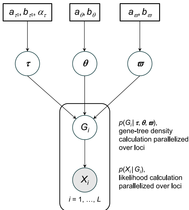
Fig. 2 | Directed Acyclic Graph (DAG) representation of the MSC-M model.
