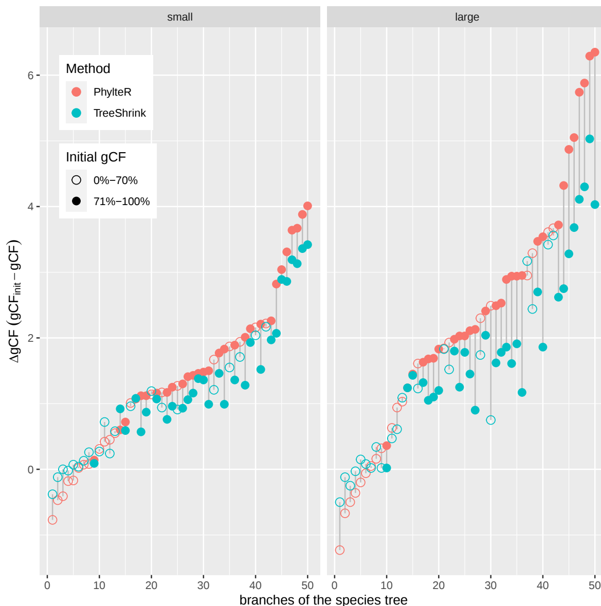
Fig. 7. Effect of filtering outliers in gene trees on the gCF of each branch of the Carnivora species tree. The gain in concordance ( \Delta\text{gCF} , y-axis) is plotted for each branch of the species tree (dots), separating PhylteR (pink) and TreeShrink (blue). Branches are ordered by increasing \Delta\text{gCF} for the PhylteR outliers. The results for the two collections of outliers (small and large) are displayed side by side.
