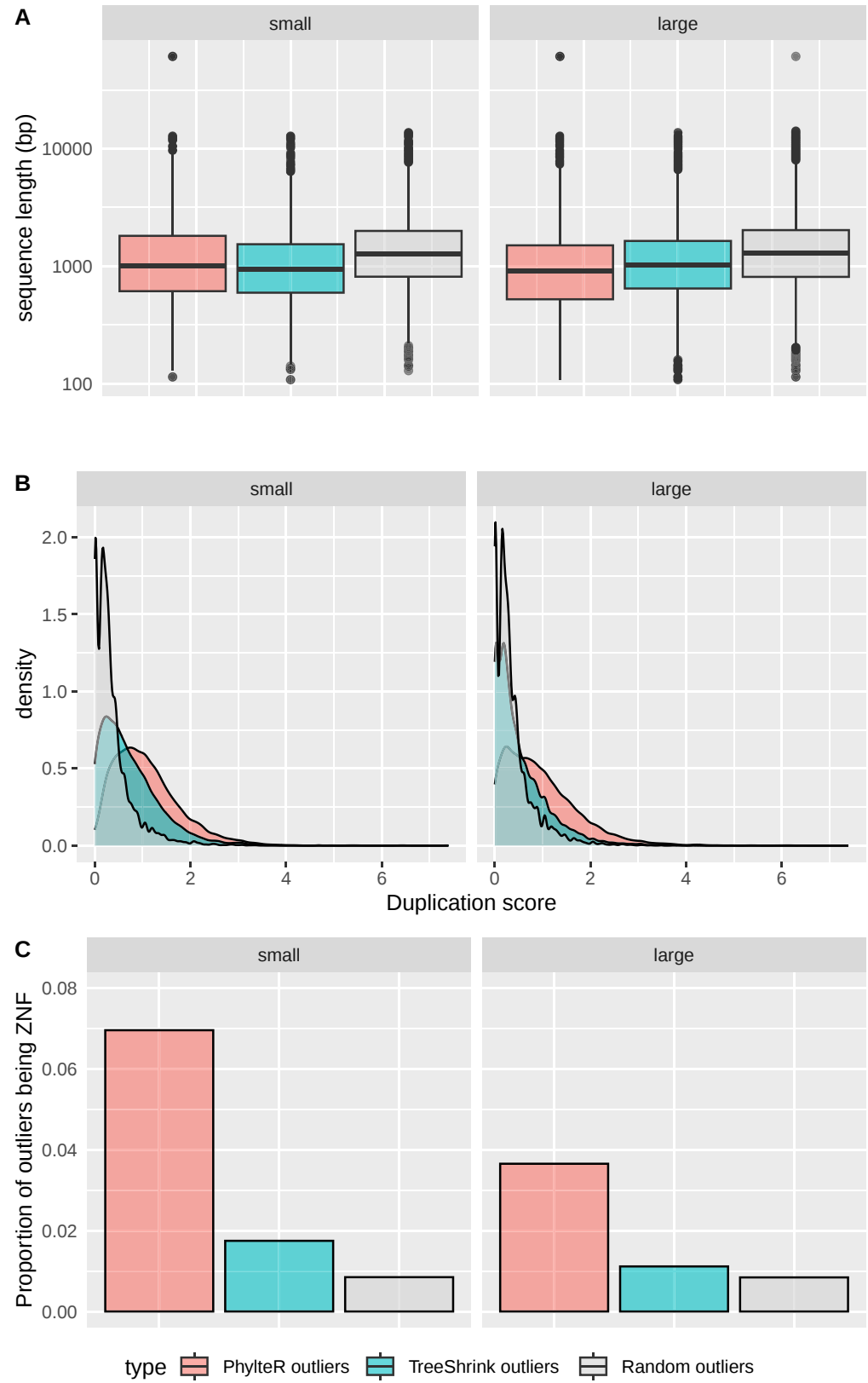
Fig. 5. Comparison of distribution values between outliers detected by PhylteR, by Tree Shrink, or randomly sampled, for three features associated with outlierness in phylogenomic datasets. a) Distribution of the length (in bp) of the sequence outliers identified by each method. A log scale is used for the y-axis. b) Distribution of duplication scores (normalized number of duplications experienced by each sequence) for the outliers identified by each method. c) Proportion of outliers being members of the KRAB-ZNF protein family for the outliers identified by each method. The two collections of outliers (small and large) are compared in each case (left and right on each panel).
