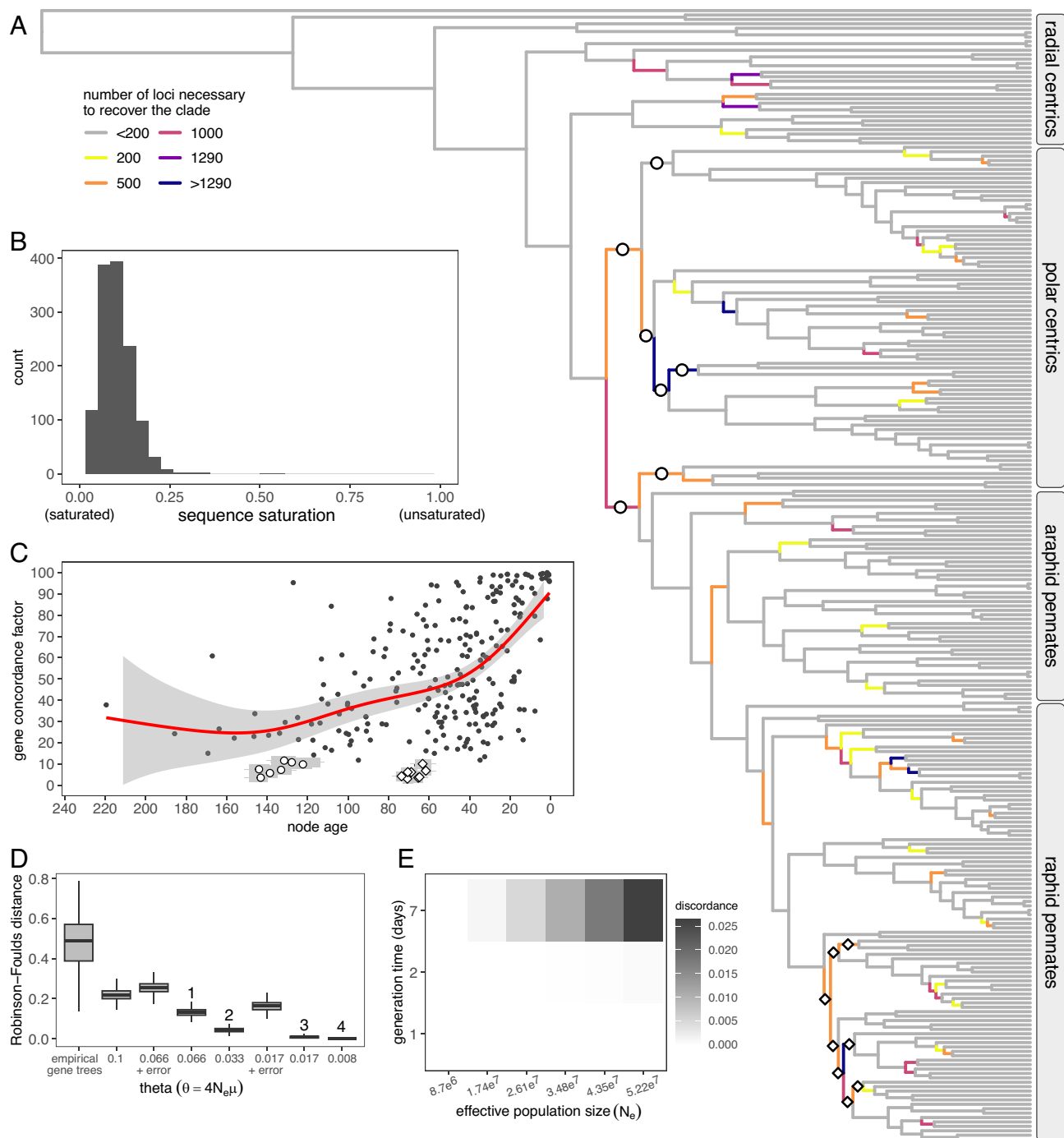
Fig. 3. The rapid radiations of polar centric and raphid pennate diatoms were marked by low gene concordance and low phylogenetic signal. (A) Species phylogeny with branches colored by the amount of data necessary to resolve each branch across simulated datasets. Most branches were consistently resolved with <200 loci, but some were unresolvable with 1,290 loci. (B) Sequence saturation across 1,290 loci, calculated as the slope of a regression between pairwise patristic distances and uncorrected genetic distances. (C) Gene concordance factor for each node in the species tree. Nodes with open circles or diamonds correspond to identically marked nodes in panel (A); gray bars represent 95% CI around age estimates; the red line indicates the fit of a generalized additive model. (D) Average distance (discordance) between the species tree and empirical gene trees ( \bar{x} = 0.48 ) far exceed expected levels based on coalescent simulations across a range of plausible values for \theta , parameterized with values from diatoms ( Fragilariopsis [1] and Phaeodactylum [3]), green algae ( Chlamydomonas [2]), and coccolithophores ( Gephyrocapsa [4]). (E) Average discordance between the species tree and empirical gene trees ( \bar{x} = 0.48 ) far exceeded discordance levels with gene trees simulated across a range of realistic values for effective population size and generation time.
