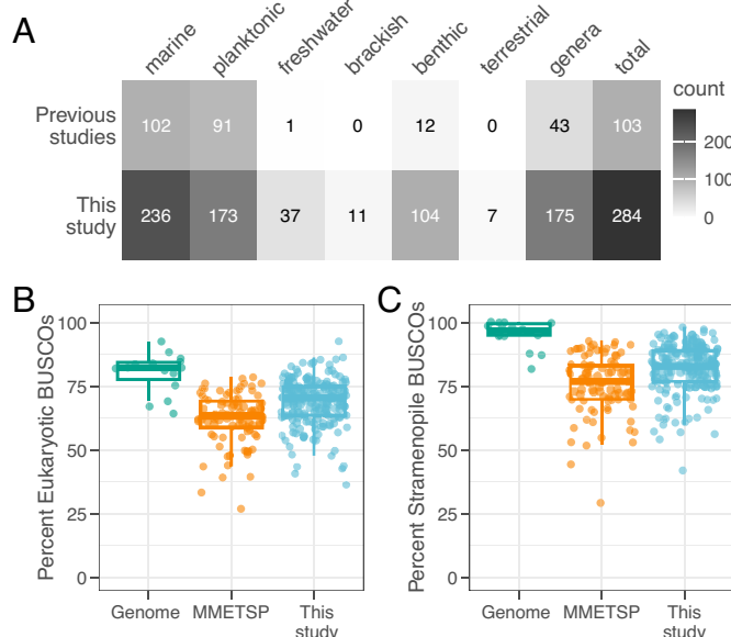
Fig. 1. High-quality transcriptomes from ecologically and phylogenetically diverse diatoms. Numbers represent total diatom strains, most of which are distinct species (A). Transcriptomes recovered a large percentage of conserved eukaryotic (B) and stramenopile (C) orthologs (BUSCOs). The estimated completeness of newly sequenced transcriptomes compared favorably to reassembled diatom transcriptomes from the MMETSP (23).
