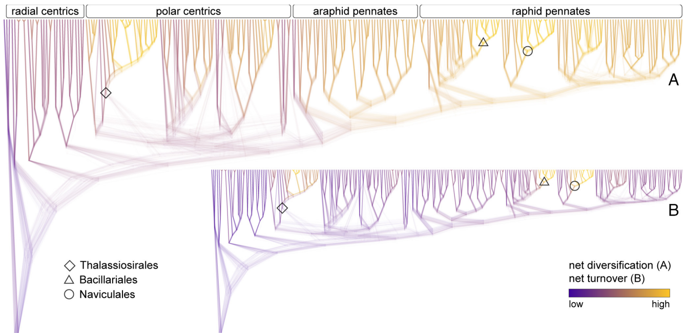
Fig. 4. Species diversification and turnover are lowest in radial centric diatoms and highest in pennate diatoms. (A) Three pulses of net diversification (speciation minus extinction) occurred in marked lineages. (B) Net turnover (speciation plus extinction) was also highest in Bacillariales and Naviculales but was sensitive to tree topology in Thalassiosirales. The analysis was run on 100 bootstrap trees that captured topological uncertainty within polar centrics and raphid pennates.
