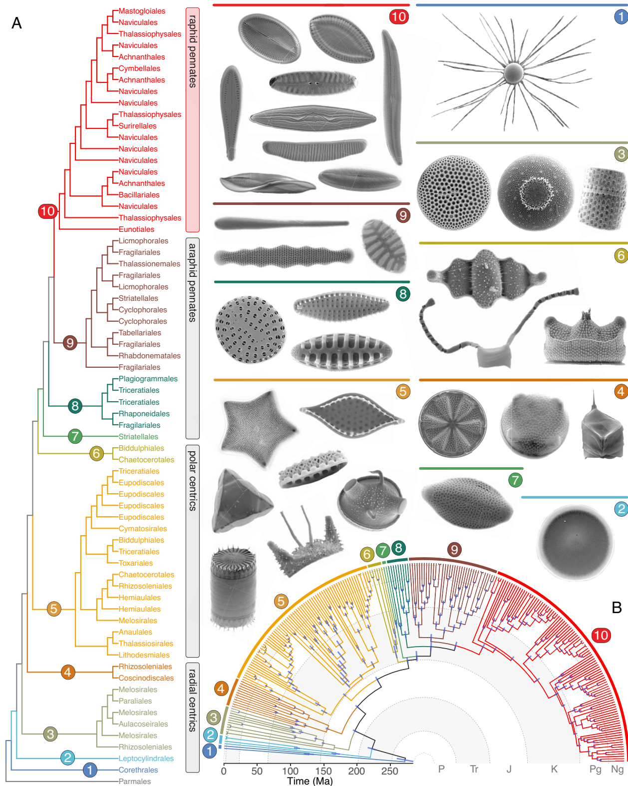
Fig. 2. The diatom tree of life. Relationships are based on maximum likelihood analysis of 240 genes and 171,434 amino acids under the LG+PMSF(C20)+F+G model. Ten numbered clades are highlighted to facilitate discussion. (A) Order-level phylogeny with major groups identified by common name. (B) Time-calibrated phylogeny. Node bars represent CI of divergence time estimates. Geologic periods are indicated as: P (Permian), Tr (Triassic), J (Jurassic), K (Cretaceous), Pg (Paleogene), and Ng (Neogene). Scanning electron microscope images show representative diatom species. Fully labeled phylogram and chronogram figures are available as SI Appendix, Figs. S5 and S6 .
