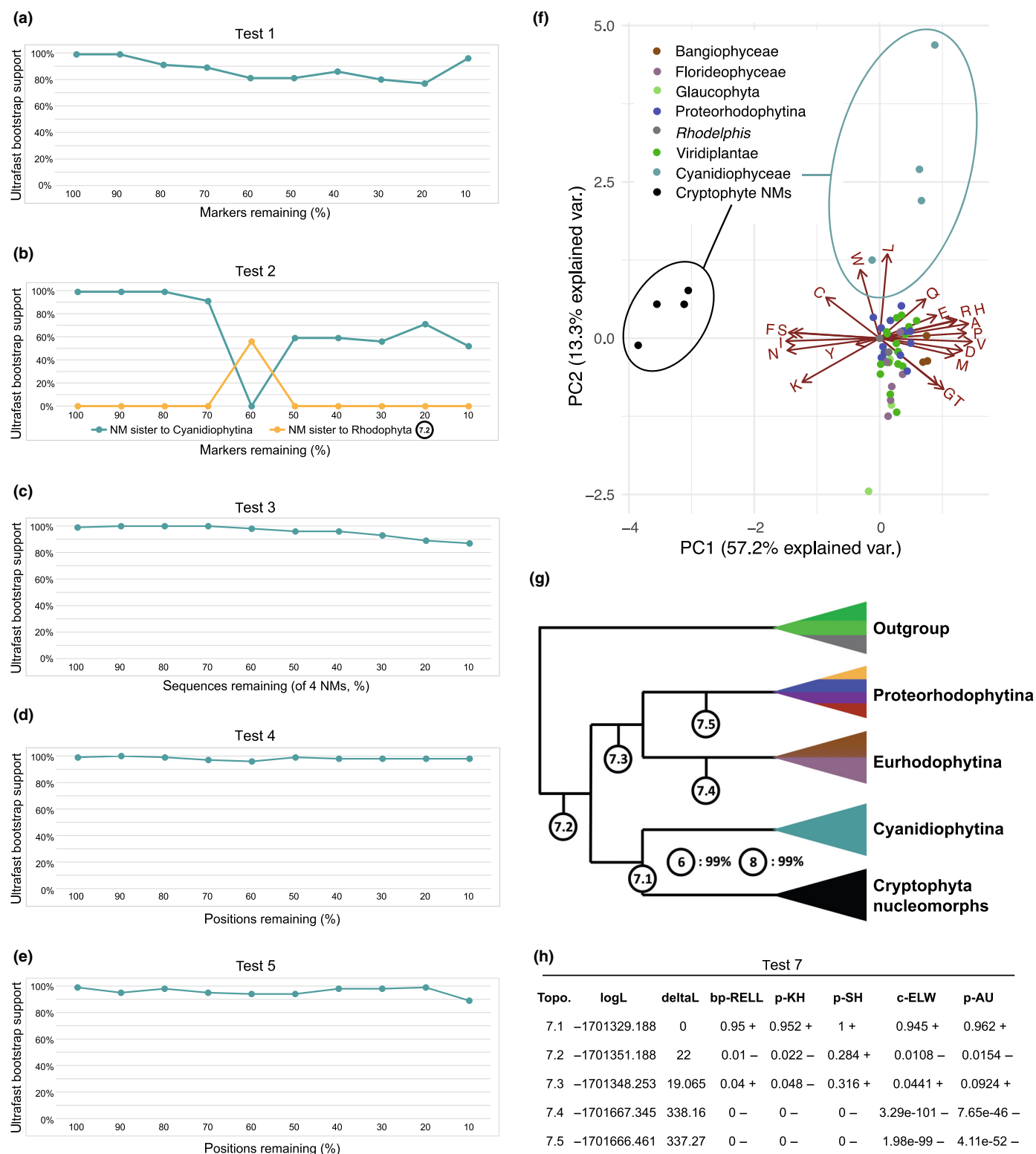
Fig. 2 Results of the topology robustness tests 1 to 8. (a–e) Changes in ultrafast bootstrap support for the sister relationship between cryptophyte NMs and Cyanidiophytina or alternative topologies as calculated based on reduced supermatrices in tests 1–5. (f) Principal component analysis of the taxa used in the phylogenetic analyses based on the amino acid composition of their sequences. (g) Simplified schematic representation of the alternative placements of cryptophyte NMs used in test 7 and ultrafast bootstrap support for the sister relationship between cryptophyte NMs and Cyanidiophytina as calculated based on modified supermatrices in tests 6 and 8. (h) Results of approximately unbiased topology tests (test 7).
