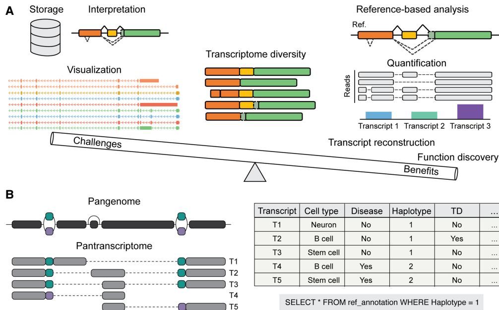
Figure 3. Genome annotation of transcriptome diversity. (A) Benefits and challenges of annotating the transcriptome diversity revealed by long-read sequencing methods. Challenges include storage, interpretation, and visualization of vast amounts of transcripts and are outweighed by the benefits of using a comprehensive reference for accurate gene quantification, transcript reconstruction, and function discovery among others. (B) Redefining the annotation paradigms. Defining haplotype-specific pantranscriptomes aligns with current pangenome efforts to describe genome diversity. Extensive meta-data annotation of the wealth of data provided by LRS allows inclusion and reference customization via subsetting to accommodate diverse analysis scenarios.
