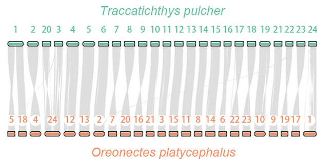
Fig. 2 Synteny analysis of the chromosomes between Traccatichthys pulcher and Oreonectes platycephalus . Unplaced: sequences that could not be anchored to any known chromosome.
