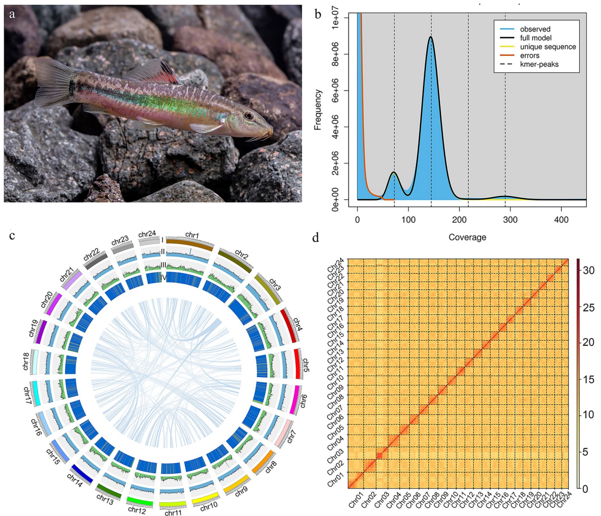
Fig. 1 The characteristics of Traccatichthys pulcher morphology and genome. (a) Morphological characters of Traccatichthys pulcher used for genome sequencing (photoed by Hao-Jun Chen). (b) GenomeScope k -mer analysis ( k = 19 ) of whole-genome sequencing reads. (c) The circos plot of genomic features: arranged from outside to inside, (I) 24 chromosomes assembly; (II) GC density; (III) TE density; (IV) gene density, and links of intragenomic syntenic blocks within 100 Kb sliding windows. (d) The Hi-C heatmap of chromosome interaction, Chr1-Chr24 is an abbreviation for 24 chromosomes. The abscissa and ordinate represent the order of each bin on the corresponding chromosome. The color from light to dark indicates the strength of the interaction from low to high.
