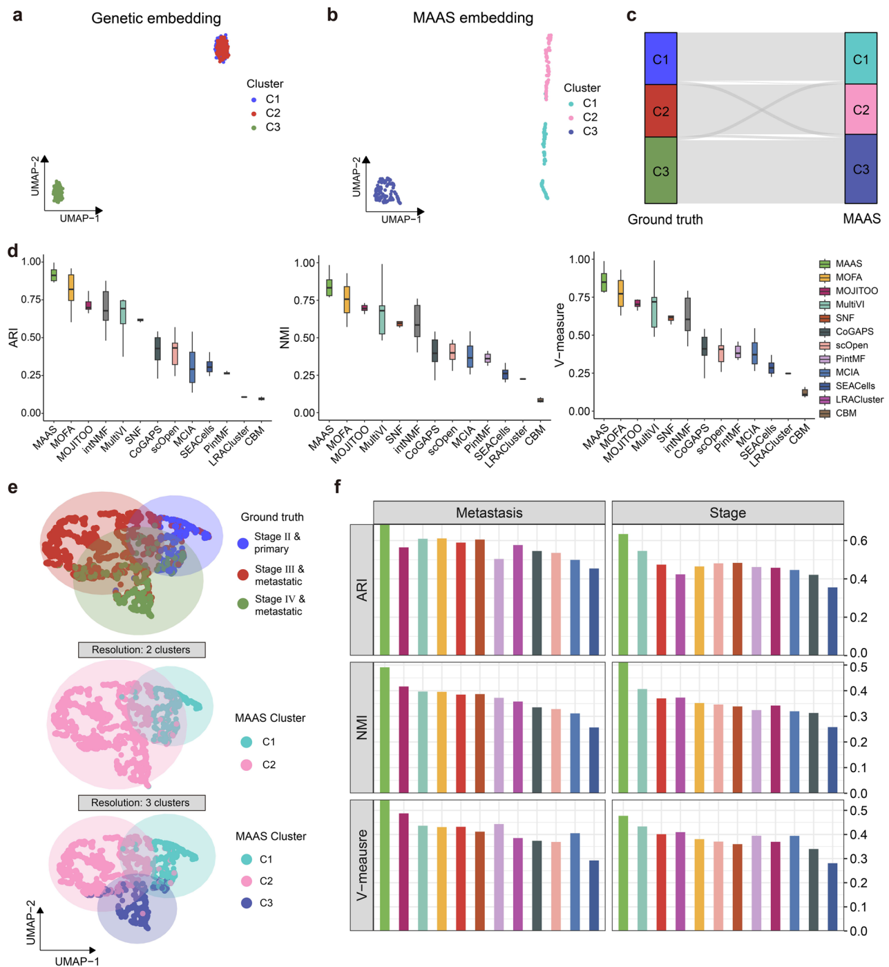
Fig. 2 Benchmarking analysis of tumor subpopulation identification. a UMAP embedding based on genetic features of three subpopulations. b UMAP embedding based on MAAS latent factors for the three identified subpopulations. c Consistency of cell distribution across the three subpopulations when comparing ground-truth to MAAS results. d Consistency of cell distributions across four subpopulations between the ground-truth and MAAS results. e UMAP embedding based on MAAS latent factors showing three ovarian cancer samples with different metastatic status and pathological stages, and MAAS-identified clusters with distinct resolution. f Accuracy of classifying tumor cell subpopulations across different computational methods. Classification performance is evaluated based on the ability to distinguish tumor subpopulations defined by metastatic status (primary vs. metastatic tumors, left panel) or pathological stages (II, III and IV, right panel)(n)
