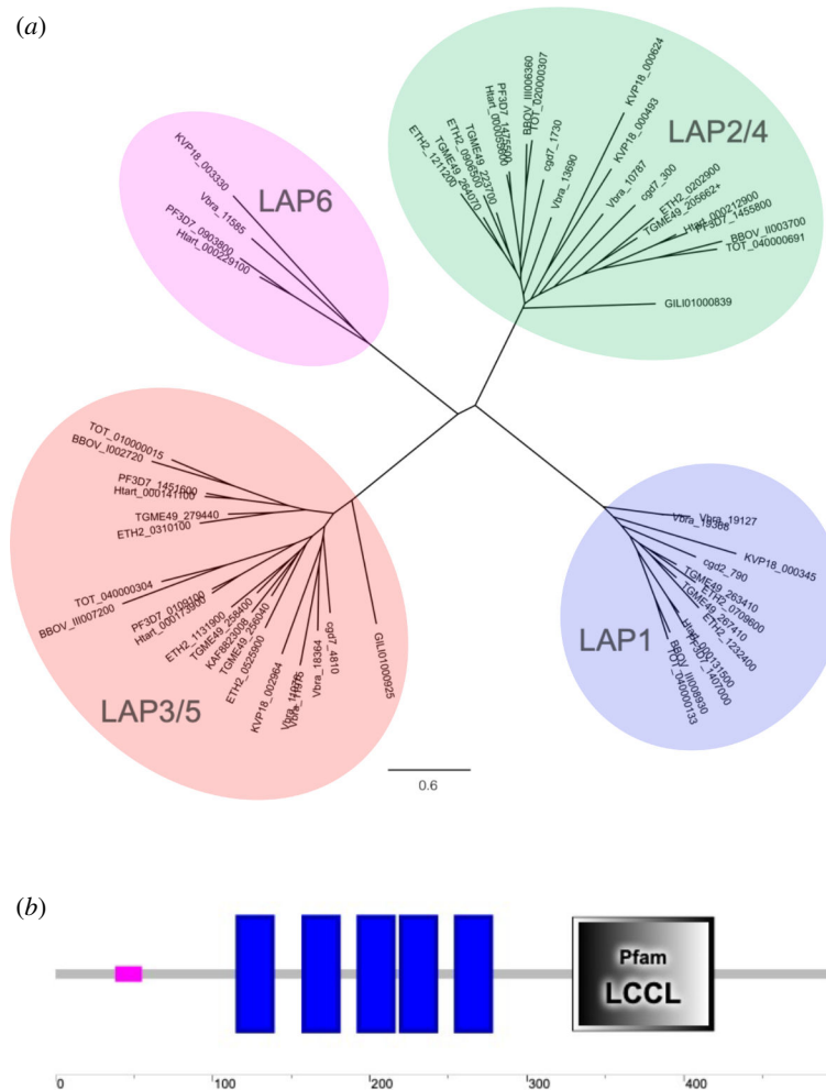
Figure 2. LAPs cluster by type. (a) Phylogeny generated from LAP1 type (blue), LAP2/4 type (green), LAP3/5 type (red) and LAP6 type (pink) amino acid sequences identified in apicomplexan, chromerid and colponemid lineages. See electronic supplementary material, table S1 for sequence details. Scale bar: substitutions per site. (b) Predicted structure of the membrane-bound LCCL-domain proteins found in chromerids. Blue rectangles represent predicted transmembrane helices (image generated in SMART).
