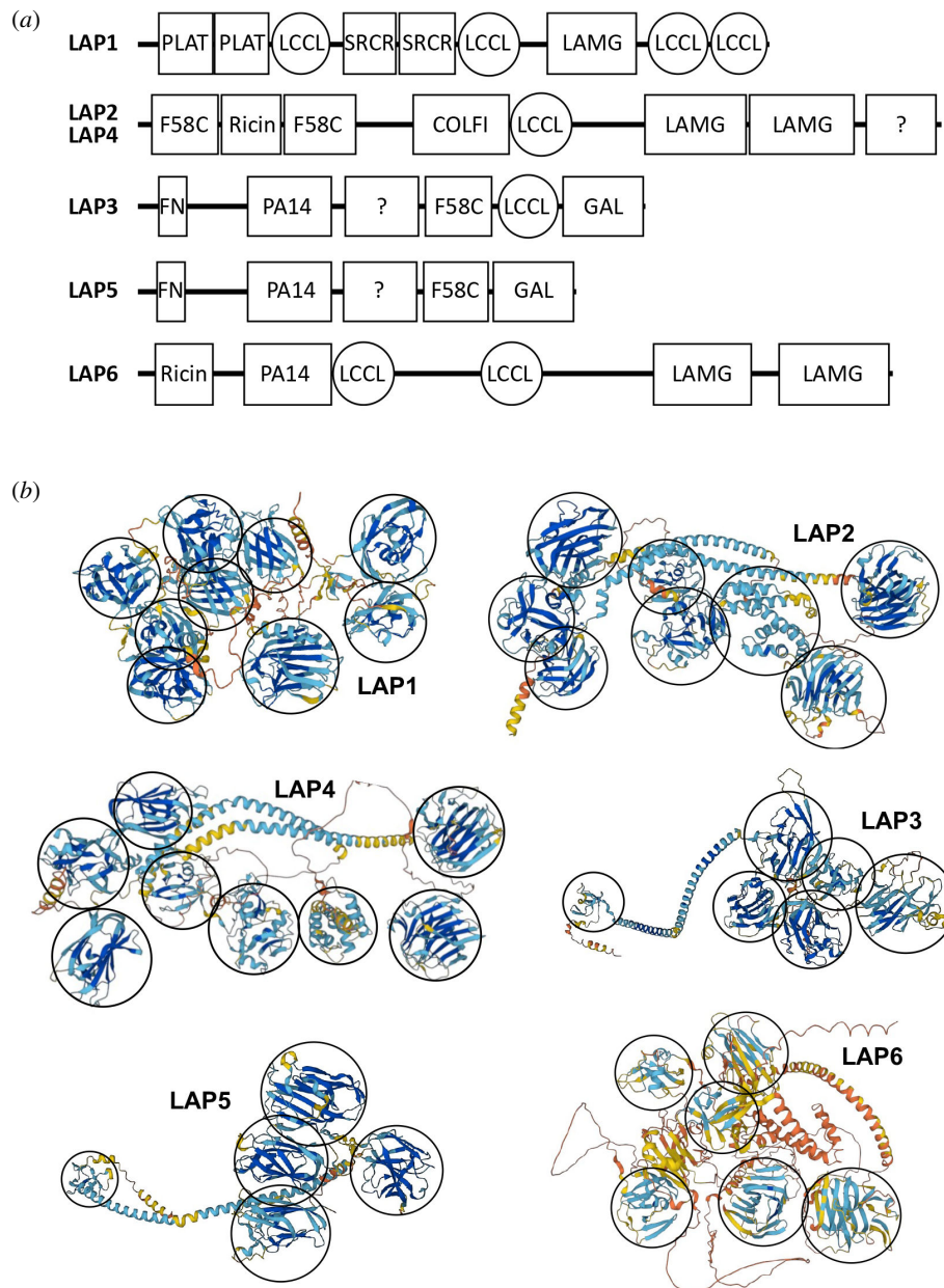
Figure 1. Predicted domain composition and organization of the LAPs. (a) Schematic linear depiction of LAP1–LAP6 with various conserved domains indicated: PLAT (polycystin-1, lipoygenase, alpha-toxin, IPR001024); LCCL ( Limulus coagulation factor C, Coch-5b2 and Lgl1, IPR004043); SRCR (scavenger receptor cysteine-rich, IPR036772); LAMG (laminin G superfamily, IPR013320, cl22861); F58C (coagulation factor V and VIII carboxy-terminal, IPR000421, related to discoidin); Ricin (ricin B lectin domain, IPR000772); COLFI (fibrillar collagen carboxy-terminal domain, SM00038, PF01410); FN (fibronectin type II domain, IPR000562); PA14 (protective antigen of anthrax toxin, IPR037524); GAL (galactose binding-like domain superfamily, IPR008979); ? (unspecified domains). (b) Predicted AlphaFold three-dimensional structure projections of Plasmodium falciparum LAP1–LAP6. Protein domains are encircled.
