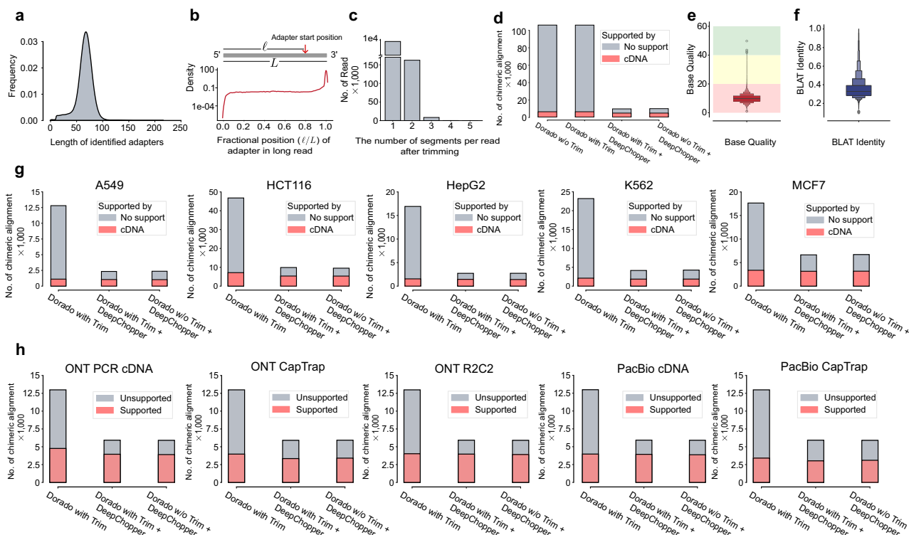
Fig. 2 | Detection of chimeric read artifacts in dRNA-seq data using DeepChopper and validation with orthogonal sequencing platforms. a Length distribution of predicted adapters by DeepChopper in VCaP dRNA-seq data. b Distribution of relative adapter position along read length in VCaP dRNA-seq data. Grey rectangle represents a long read from 5' to 3'. Relative position is calculated as the ratio of the length before DeepChopper predicted adapter start position to the total read length. c Distribution of segments per read after trimming: 1 segment indicates 3' end adapter trimmed, while 2 or more indicate internal adapters trimmed. d Chimeric alignments (in thousands) for VCaP dRNA-seq reads processed by Dorado with and without adapter trimming, Dorado with adapter trimming followed by DeepChopper, and DeepChopper. Gray bars represent unsupported chimeric alignments (likely artifacts); pink bars represent cDNA-supported chimeric alignments (biological events). DeepChopper-involved methods reduce chimeric alignments not supported by direct cDNA sequencing. e Base quality score distribution for internal adapter sequences identified by DeepChopper. Background colors indicate quality thresholds: green (Q > 20), yellow (Q = 10–20), red (Q < 10). Enhanced box plot shows median (center line, 9.80), interquartile
