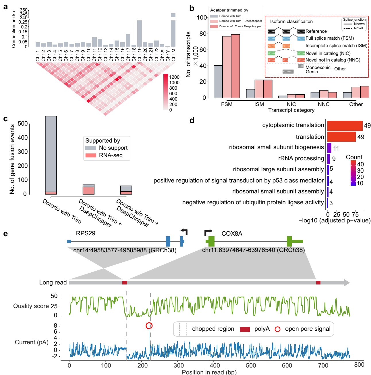
Fig. 3 | Characterization of dRNA-seq chimera artifacts and their impact on downstream analysis in VCaP cells. a The upper bar plot shows the number of chimeric connections per kilobase across chromosomes, highlighting higher chimeric activity in Chr 19 and Chr M. The lower heatmap visualizes interchromosomal connections, with intensity indicating the count of connections between different chromosomes. b The bar plot shows the number of transcripts (in thousands) across different isoform classification categories. DeepChopper-processed reads result in a higher number of transcripts compared to Dorado-trimmed reads. The inset details the isoform classification scheme. c Detected gene fusions from Dorado adapter-trimmed reads and DeepChopper-processed reads. Gene fusions identified from short-read RNA-seq were used to validate fusion events detected
