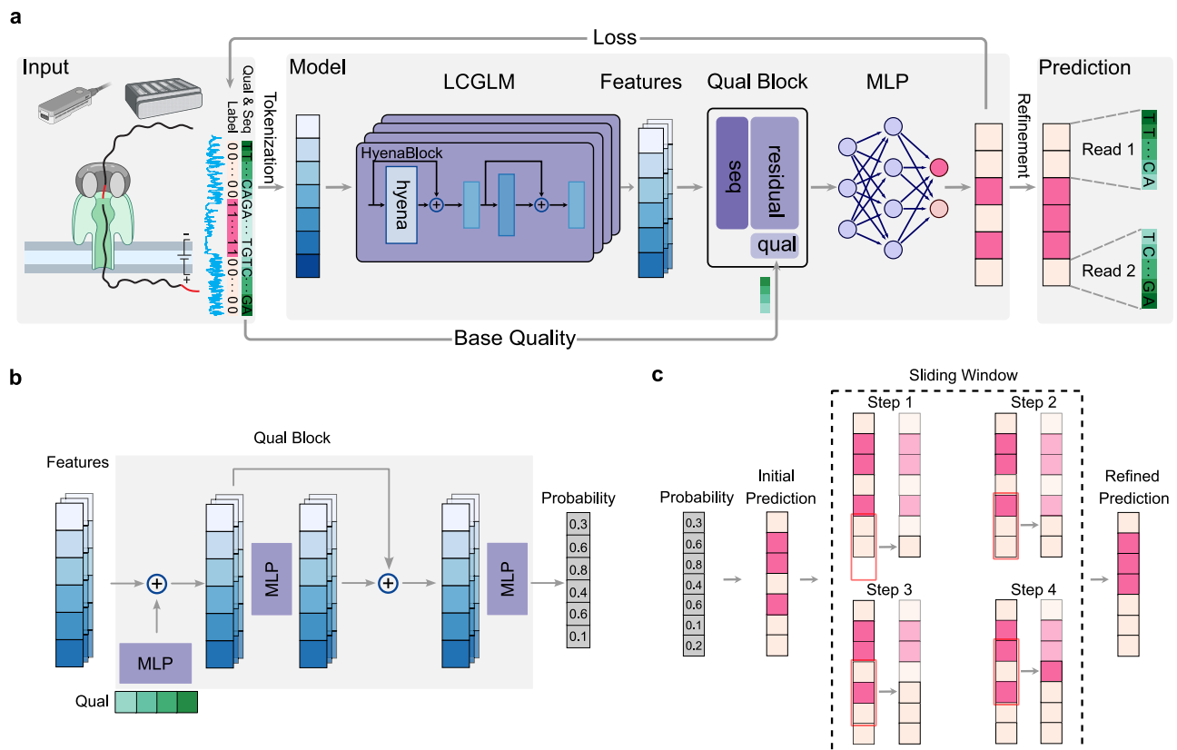
Fig. 1 | DeepChopper architecture and methodology. a Overview of the DeepChopper model. Raw sequences are first tokenized into vectors and processed by HyenaDNA, a long-context genomic language model (LCGLM), to generate embedding features. These features are integrated with base quality information in the quality block to produce per-token probability scores. A refinement strategy further optimizes the predictions. Created in BioRender. Guo, Q. (2026) https://BioRender.com/zlls0nk . b Architecture of the quality block. The block combines a multi-layer perceptron (MLP) (purple) with a residual connection to
