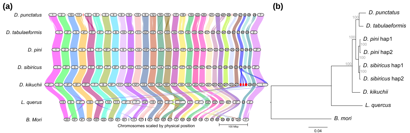
Figure 5 Comparative syntenic and phylogenetic analysis of seven lepidopteran genome assemblies. a) The syntenic riparian plot. Chromosome numbers are those provided by the corresponding NCBI projects. Unplaced scaffolds are marked by red fill. b) The phylogenetic trees based on single-copy orthologous proteins. The dendrogram also includes both partially phased haplotypes from the diploid assemblies of D. sibiricus and D. pini genomes. The trees are rooted using B. mori as outgroup. Numbers show node bootstrap support values. The trees were generated on partitioned data using IQ-TREE maximum likelihood inference with 10,000 bootstraps and WAG substitution model.
