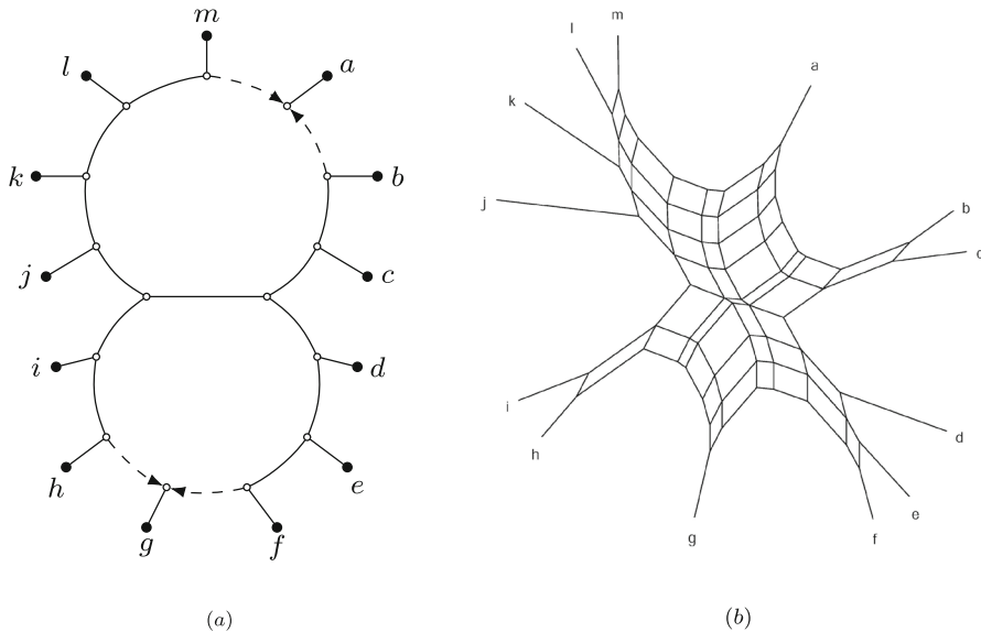
Fig. 12 Left: An outer-labeled planar, galled, level-2, semi-directed bloblet network N on leaf set X = \{a, \dots, m\} . Right: The splits graph of the pairwise NANUQ distances d_N of the network N , obtained with NEIGHBOR-NET (Bryant and Moulton 2004)
