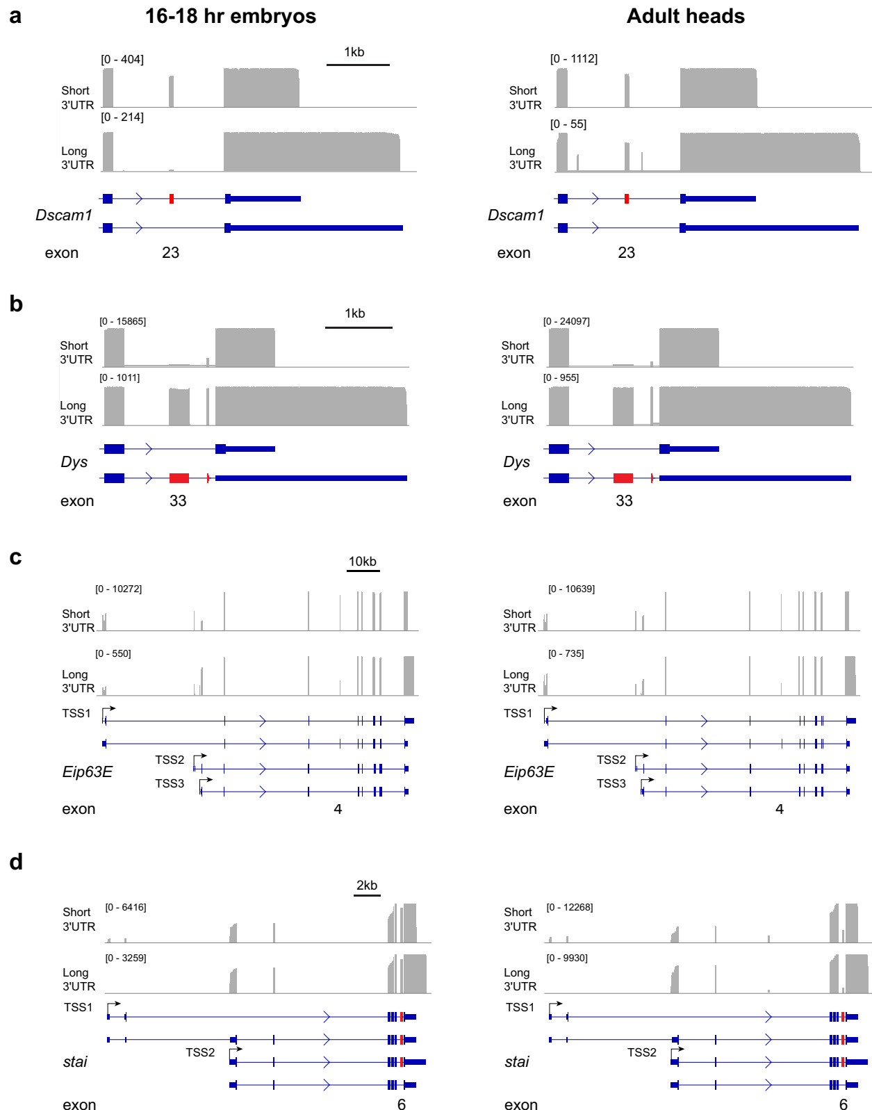
Fig. 4 | PL-Seq tracks of genes exhibiting 3'UTR connected CE splicing. Left side shows 16–18 hr embryos and right side shows adult heads. a Dscam1 , b Dys , c Eip63E , and d stai . For quantification of CE PSI see Fig. 3 and supplementary Fig. 5.
