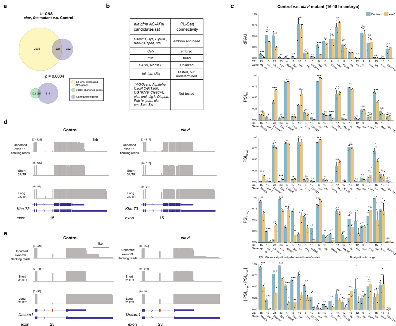
Fig. 6 | ELAV loss of function deregulates 3'UTR connected CE splicing. a Fisher's exact test (two-sided) shows 3'UTR shortening genes in elav, fne mutants are significantly associated with regulated CE events when comparing RNA-Seq data from L1 CNS elav, fne mutants with controls 9 . b List of the 29 AS and APA regulated genes in elav, fne mutants with PL-Seq verification information for 3'UTR connected CE splicing. c dPAU, PSI from all transcripts (PSI All ), short (PSI Short ) and long (PSI Long ) 3'UTR isoforms, and CE splicing difference between short and long 3'UTR isoforms (|PSI Long - PSI Short |) compared between control and elav mutant embryos using PL-
