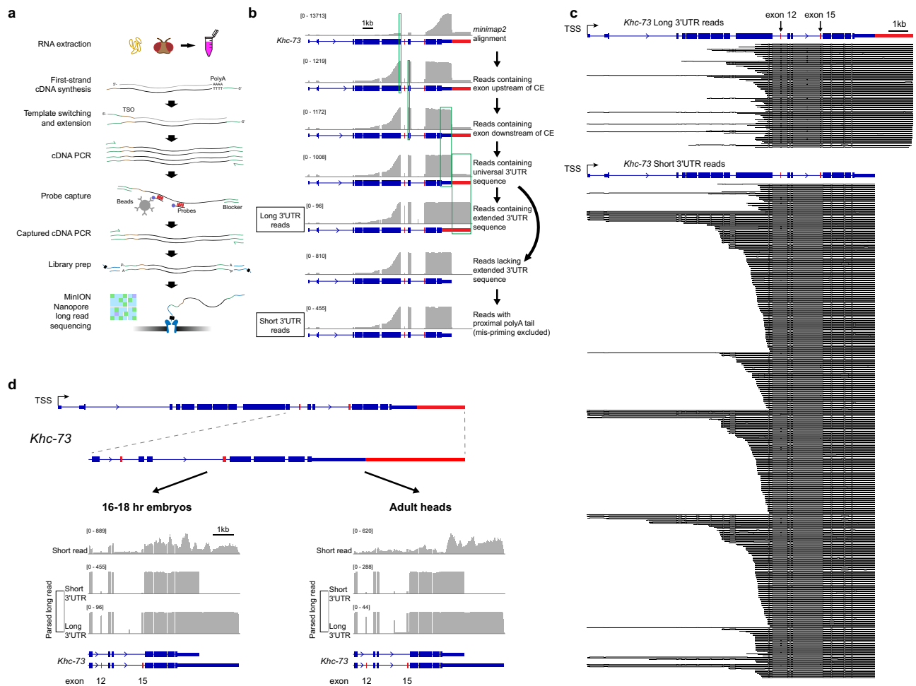
Fig. 2 | PL-Seq library preparation and data processing workflow. a Illustration showing PL-Seq library preparation. b Filtering of reads and parsing to long and short 3'UTR isoforms demonstrated on the Khc-73 gene. Reads aligned to Khc-73 are filtered to ensure that they contain upstream and downstream constitutive exons of each specific CE event, and the universal 3'UTR sequence and then parsed to long
