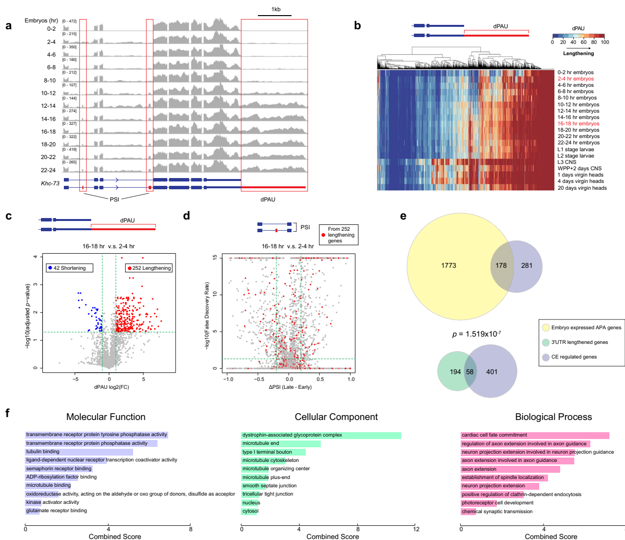
Fig. 1 | APA and AS analysis of short-read RNA-Seq data across development and tissues in Drosophila . a Short-read RNA-Seq data 47 shows coordinated inclusion of CEs with 3'UTR lengthening during embryonic development for the Khc-73 gene. b Distribution of Distal PolyA Site Usage (dPAU) values from different embryonic stages and larval/adult tissues. The value of dPAU falls into a range from 0 (no distal polyA site usage) to 100 (exclusive distal polyA site usage). c dPAU compared between late-stage embryos (16–18 hr) and early-stage embryos (2–4 hr). p values are calculated from two-tailed t-test, and then adjusted using FDR. Blue represents FDR adjusted p < 0.05 and FC < 0.5 while red represents adjusted p < 0.05 and FC > 2 . FC, fold change. d Change in PSI compared between late-stage
