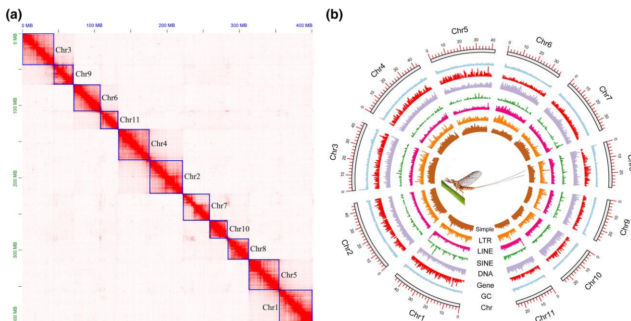
Fig. 1. a) Heatmap of interaction frequency of genomic fragments of P. youi . b) Circo map depicting the characters of the P. youi genome.
